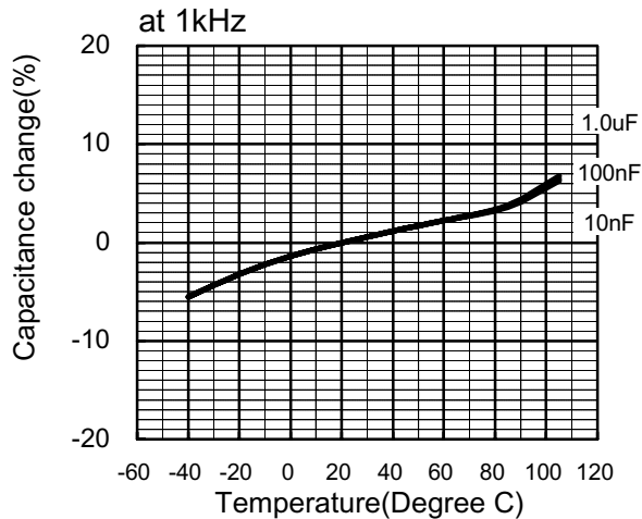
Temperature Characteristics
